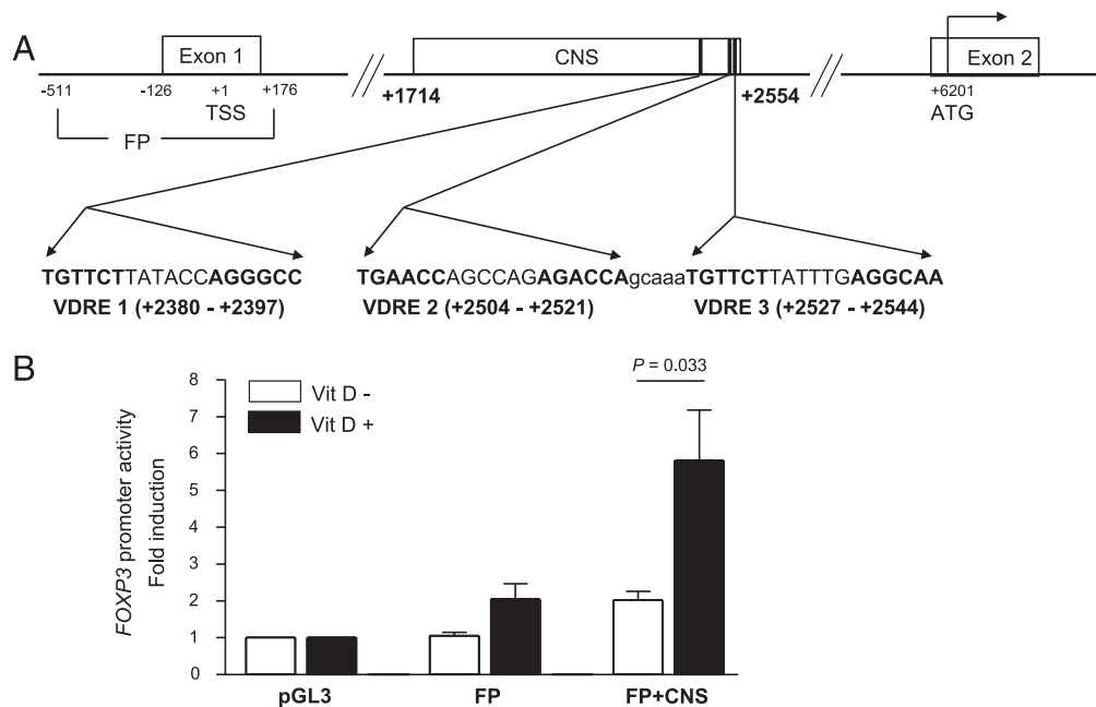
FIGURE 1. Identification of putative VDREs in the intronic CNS region +1714 to +2554 of the human FOXP3 gene that increases the FOXP3 promoter activity in response to 1,25(OH) 2 VD 3 . (A) The locations and sequences of three putative VDREs in the intronic CNS region +1714 to +2554 of the human FOXP3 gene. The sequences of the putative VDREs are in boldface type. (B) The CNS region +1714 to +2554 increases the human FOXP3 promoter (FP, -511 to +176) activity in the presence of 1,25(OH) 2 VD 3 , anti-CD3/CD28 Abs, and IL-2 as measured by luciferase reporter assay. Human primary CD25 - CD4 + T cells were stimulated for 5 d with anti-CD3/CD28 Abs and IL-2 (25 ng/ml) in the presence or absence of 1,25(OH) 2 VD 3 (Vit D, 10 nM) and transfected with pGL3 basic vector (PGL3), vector with an insert containing the FOXP3 promoter (FP), or vector containing the FOXP3 promoter and the CNS region +1714 to +2554 (FP+CNS). Cells were additionally incubated for 2 d in the presence of the same stimulation, with or without 1,25(OH) 2 VD 3 . Luciferase activity was measured and normalized against Renilla activity. Data represent the means ± SEM from six independent experiments.
