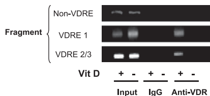
FIGURE 3. Detection of VDR binding to VDRE1 and VDRE2/3 in the CNS region +1714 to +2554 of the human FOXP3 gene using a ChIP assay. Human CD25 - CD4 + T cells were treated for 5 d with or without 1,25(OH) 2 VD 3 (Vit D, 10 nM) in the presence of anti-CD3/CD28 Abs and IL-2. Cell lysates were immunoprecipitated with anti-VDR Abs or control IgG. Immune complexes were collected, and PCR analysis was performed to determine the presence of VDRE1, VDRE2/3, and non-VDRE (-145 to +5, control) regions against input DNA. Representative data are from three independent experiments.
