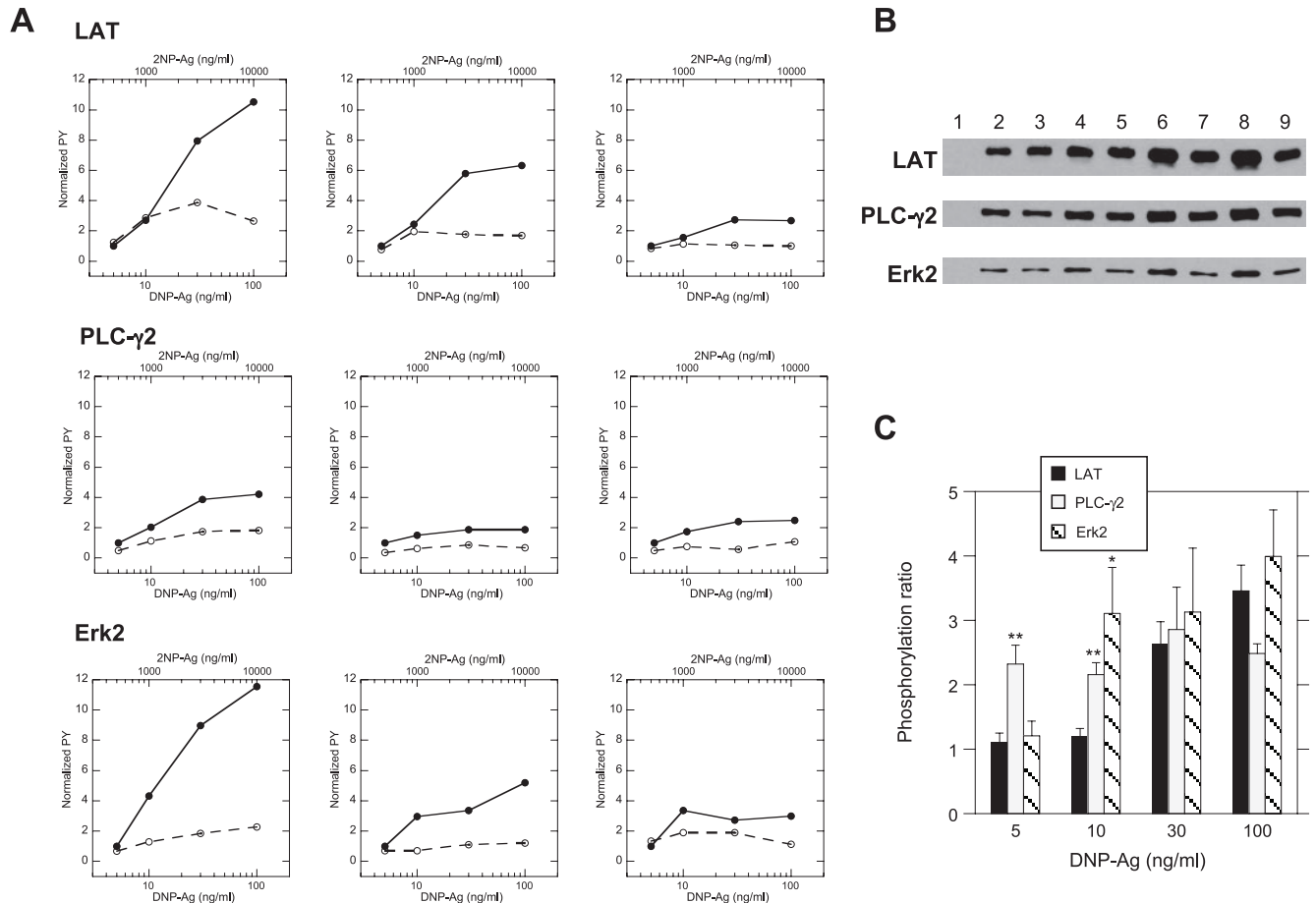
FIGURE 1. Relative levels of phosphorylation induced by DNP-Ag and a 100-fold higher concentration of 2NP-Ag for a range of ligand concentrations. A , Ligand dose-response curves for LAT, PLC- \gamma 2, and Erk2 phosphorylation stimulated by DNP-Ag (solid lines, filled circles, concentration on lower x -axis) and a 100-fold higher concentration of 2NP-Ag (dashed lines, open circles, concentration on upper x -axis). Each column contains data from a single experiment. LAT and PLC- \gamma 2 phosphorylation are detected at 3 min and Erk2 phosphorylation is detected at 5 min following stimulation. B , Representative Western blots used to generate the data plotted in A . Lane 1, control (resting), lanes 2, 4, 6, and 8: DNP-Ag at 5, 10, 30, and 100 ng/ml, respectively; lanes 3, 5, 7, and 9: 2NP-Ag at 500, 1000, 3000, and 10,000 ng/ml, respectively. C , Ratios of phosphorylation obtained for each dose combination tested. Values plotted are the average of the three experiments shown in A at each concentration ( \pm SEM). The significance of the difference in phosphorylation at each dose combination was evaluated using a paired Student's t test (*, p < 0.05 ; **, p < 0.01 ).
